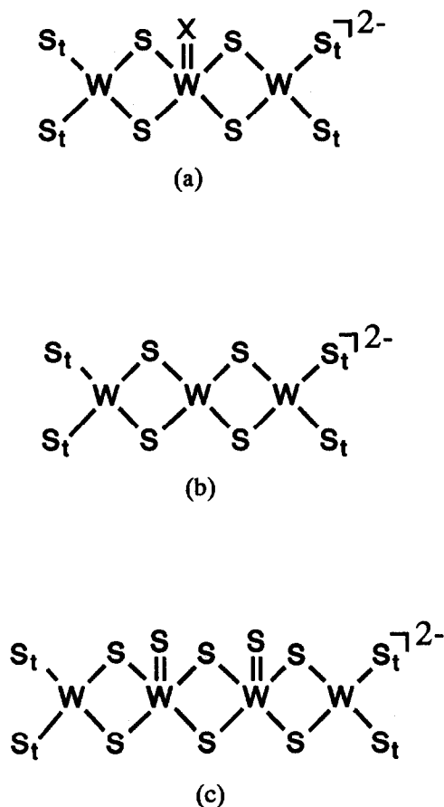
Fig. 20. Tungsten linear tri- and tetranuclear compounds with (a) [(WS_4)W(X)(WS_4)]^{2-} ( X = O, S ), (b) [(WS_4)W(WS_4)]^{2-} , or (c) [(WS_4)W(Si)(\mu-S)_2W(Si)(WS_4)]^{2-} .
