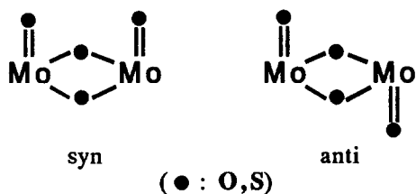
Fig. 3. Molybdenum dinuclear compounds with syn - and anti - \text{Mo}_2\text{O}_{4-n}\text{S}_n cores.
