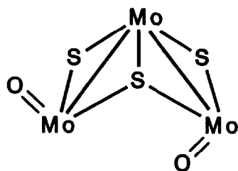
Fig. 13. Structure of the \text{Mo}_3(\text{O}_t)_2(\mu_3\text{-S})(\mu\text{-S})_2 core.
